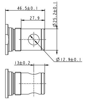
Back fixture option "1 & 2" Drawing no.: 0361129
