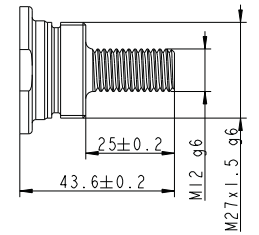
Back fixture option "5" Drawing no.: 0361126
